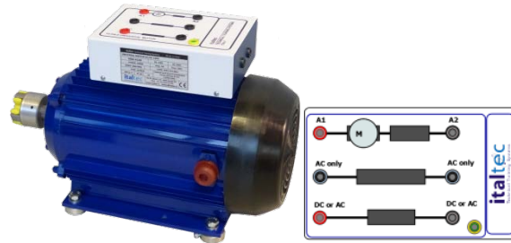
Mod.6090 Single Phase Ac Capacitor Run Motor Squirrel cage Motor Mod.6090-4 Single Phase Ac Capacitor Run Motor Squirrel cage Motor
